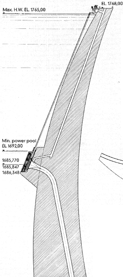
Section B-B
