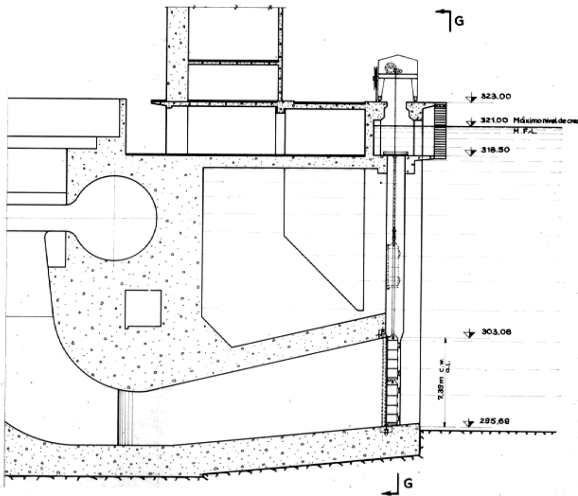
CORTE F-F SECTION F-F
