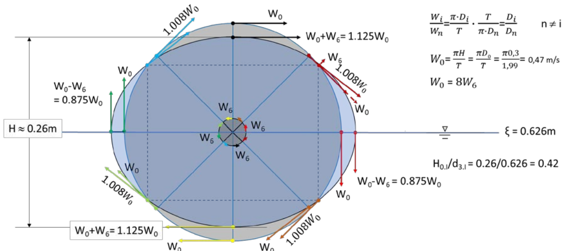
Fig.09: Graphic determination of the elliptical orbital path for a shallow sea with flat ground. Mirror axis of configuration I. Vector addition for the ratio D_{0,1}/D_{6,1} = 0.3\text{m}/0.0375\text{m} = 8/1 , which results for the still water level according to the coordinate \xi = d_{0,1} = 0.626\text{m} and the reflection of the orbital motion at \xi = -0.626\text{m} (below the ground), cf. Fig. 5. Thus, the relationship W_0 = 8W_6 applies to the circumferential velocities.
