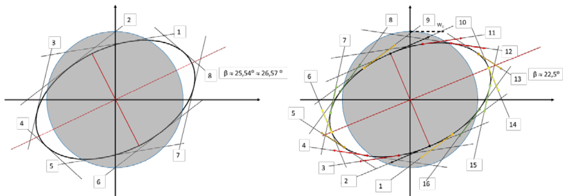
Fig.17: Comparison of only slightly different elliptical orbital paths on the surface at position d_{0,II} Left: according to the ground inclination 26.57^\circ with respect to the ground inclination also present in the hydraulic model, based on 8 phase points (Fig.13) and right with respect to the slightly different ground inclination 22.5^\circ based on 16 phase points.
