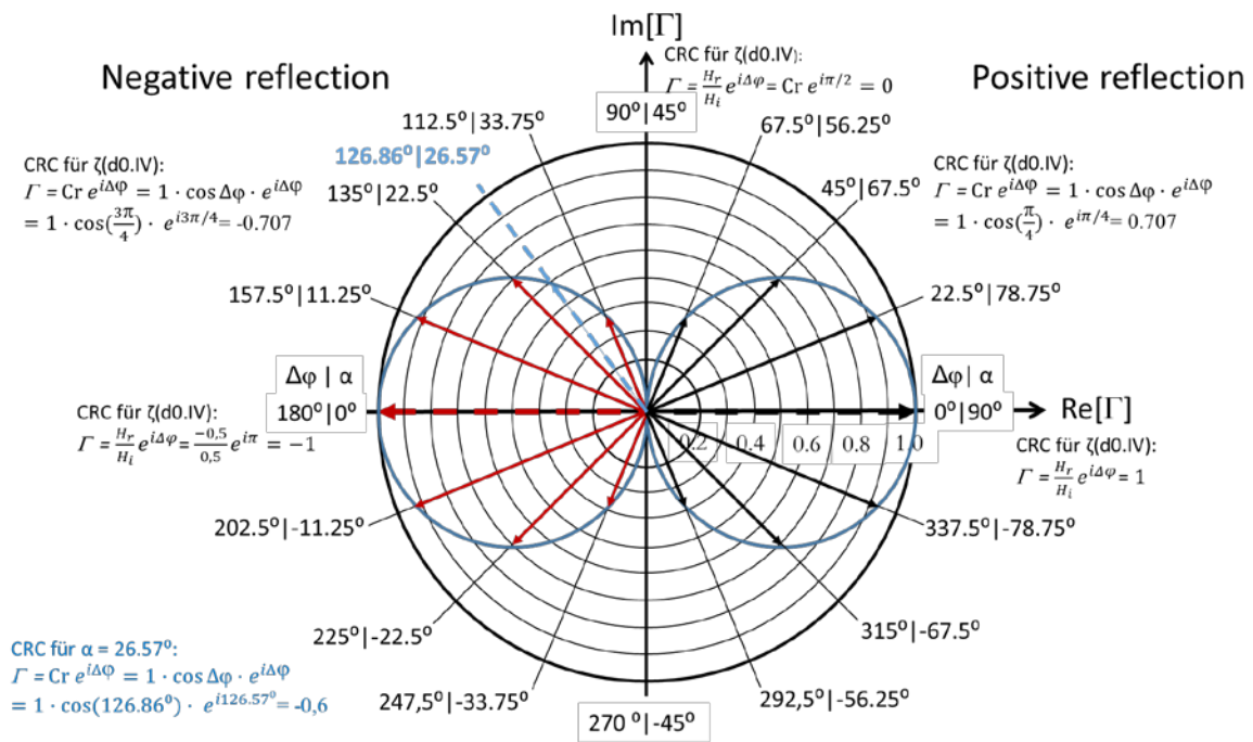
Fig. 27: Pointer diagram for the representation of complex reflection coefficients CRC \Gamma = C_r e^{i\Delta\varphi} for phase jumps 0^\circ \leq \Delta\varphi \leq 180^\circ (left value) corresponding to slope angles 90^\circ \geq \alpha \geq 0^\circ (right value) with respect to the exponentially reduced mirroring at the intersection IP of the still water level (d0.IV) with the slope in question.
