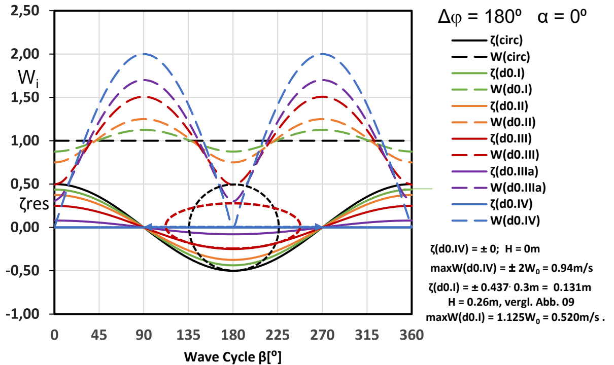
Fig. 23: Unit orbital velocity magnitudes W(d0.IV) and unit water level deflections \zeta(d0.IV) = 0 for the wave cycle of the negative Clapotis \xi ( d0.IV) = 0.0m for the mirror depth \xi = 0.0m ( d0.IV ) and of 4 partially negatively reflected waves \zeta(d0.IIIa) , \zeta(d0.III) , \zeta(d0.II) , \zeta(d0.I) , for the 4 fictitious mirror depths 0.106m, 0.212m, 0.412m and 0.626m above flat ground, as well as the above-mentioned orbital paths, see Fig. 12
