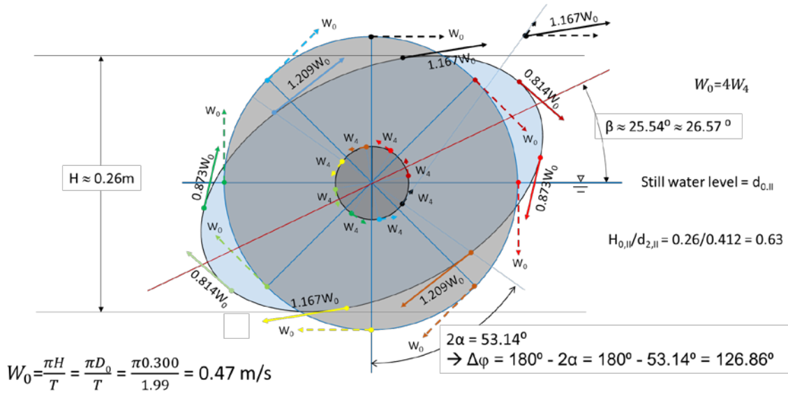
Fig. 13: Graphical determination of the elliptical orbital paths above the slope 1: n = 1: 2 , (corresponding to \alpha = 26.57^\circ ). Mirror axis of configuration II. Vector addition for the ratio D_{0,II}/D_{4,II} = 0,300\text{m}/0,075\text{m} = 4 , which results in the water level ( d_{0,II} = 0.0\text{m} ) corresponding to the coordinate \xi = 0.412\text{m} and the reflection of the orbital motion at \xi' = -0.412\text{m} (below the inclined ground), cf. Fig.12. Thus, the relationship W_0 = 4W_4 applies to the circumferential velocities on the elliptical path.
