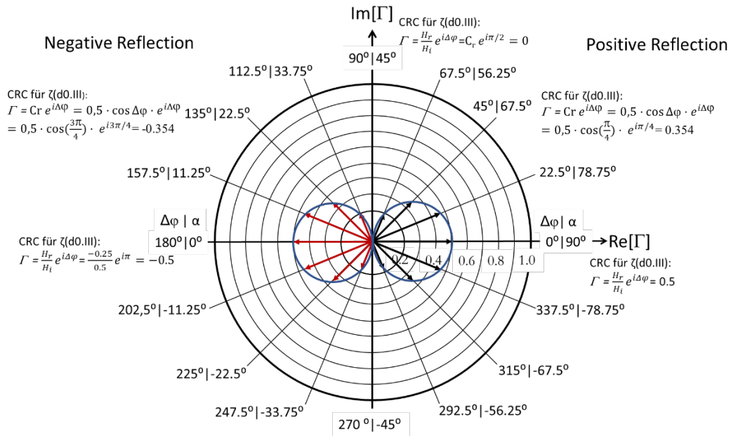
Fig.28: Pointer diagram for the representation of complex reflection coefficients CRC \Gamma = C_r \cdot e^{i\Delta\varphi} for phase jumps 0^\circ \leq \Delta\varphi \leq 180^\circ (left value) corresponding to slope angles 90^\circ \geq \alpha \geq 0^\circ (right value) with respect to the exponentially reduced mirroring at the Intersection of the still water level (d0.III) with the mirror axis III.
