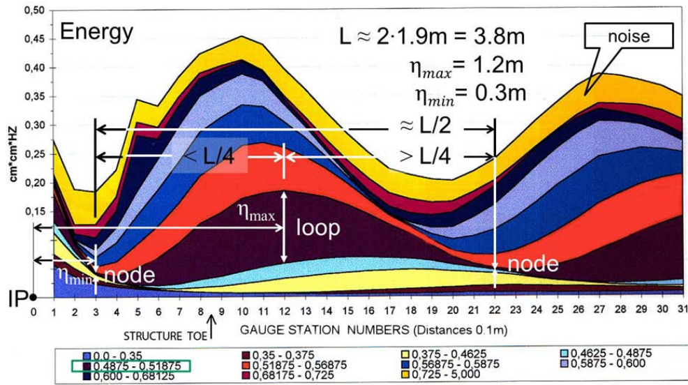
Fig.11: To determine the length L and the phase difference \Delta\varphi between incident and reflected wave using the example of the partial wave of the frequency range 0.4875\text{Hz} \leq f \leq 0.51875\text{Hz} at a flat slope 1:2. As a result of the horizontal wave asymmetry of the almost breaking waves (characterized by \eta_{\max} - \eta_{\min} < L/4 ), the formulas (10a) and (10b) provide two different results for the phase shift \Delta\varphi = 132.6^\circ > 123.2^\circ . Further explanation in (Büsching, F., 2012 [1]) or (Büsching, F., 2011 [8]).
